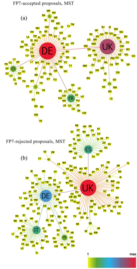
Fig. 6. Minimum Spanning Tree of (a) the network of countries involved in the FP7 accepted proposals and (b) the network of countries involved in the FP7 rejected proposals. The colour (online) of the circles representing the countries varies with respect to the degree of the node in the MST network, according to the chromatic scale shown at the bottom-right part of the figure.
